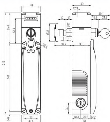
Switch FY 6•••••• with integrated control devices
