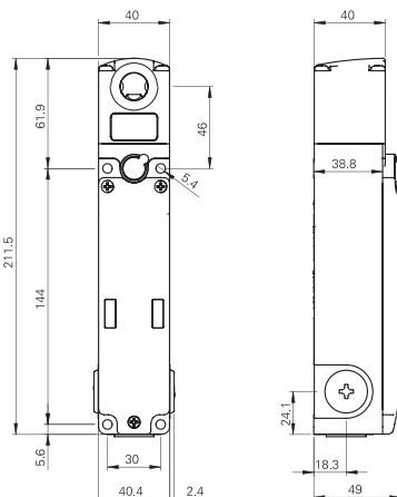
Switch NG 2D7D●●1 A
