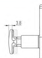
Release button travel
