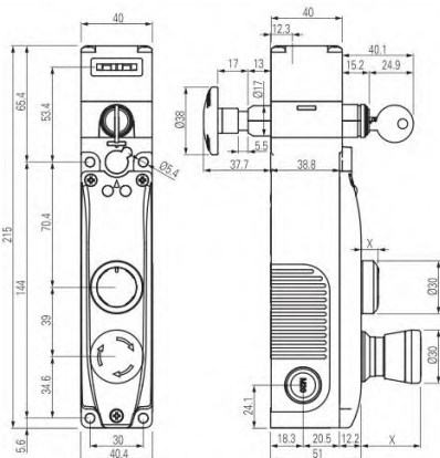
Switch FY 6•••••• with integrated control devices
