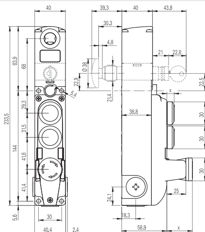
NG 2D ●●●●●● switch with integrated control devices
