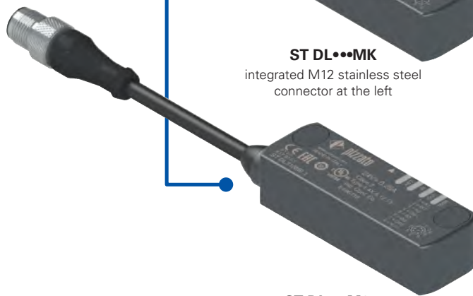
ST DL...M0.1 cable, length: 0.1 m, with M12 connector at the left
