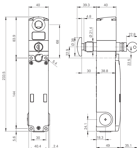
NG 2D ●●●●●● switch with integrated control devices
