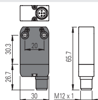
M12 connector, bottom
