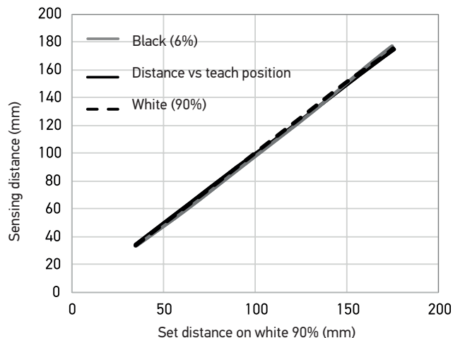
S3N-PR-5-M03-OZ (Sensing vs. Set Distance difference)
