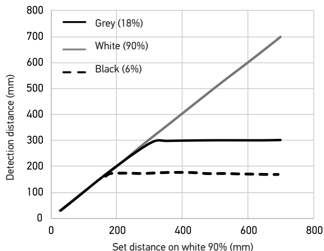
S3N-PH-*-M03-* (Black and white difference)
