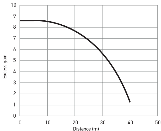
S3N-PH-*-FG*-* (Excess gain)
