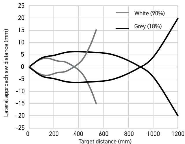
S3N-PR-*-C1*-** (Beam diagram)
