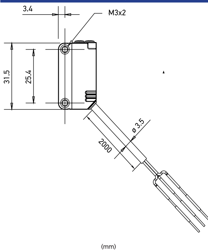
S3N-P*-2-****-** (Cable out)
