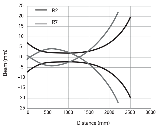
S3N-PR-*-T5*-* (Beam diagram)
