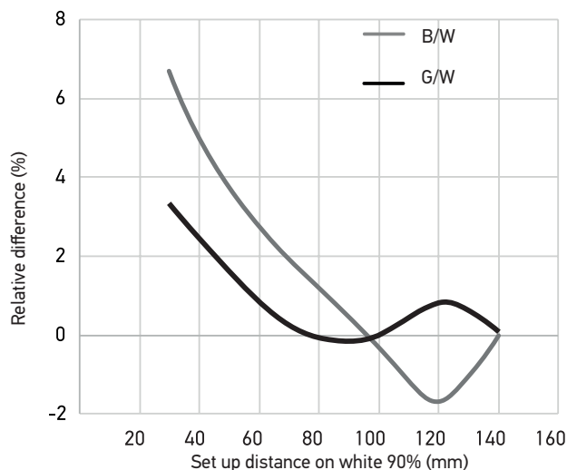
S3N-PH-*-M03-* (Black and white difference)
