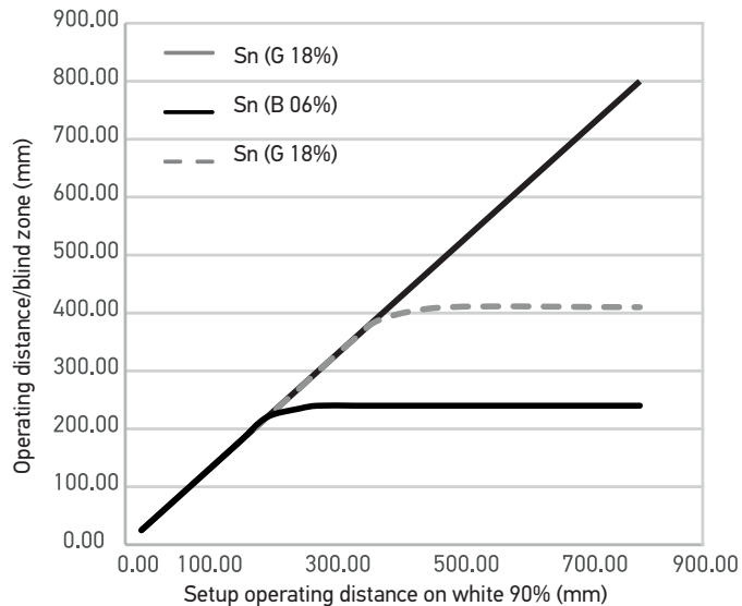
S3N-PR-*-M01-* (Operating distance)
