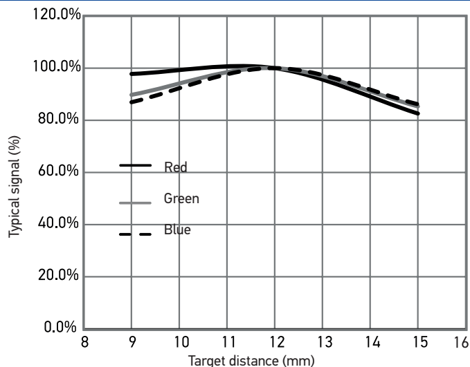
S3N-PR-*-W03-OZ (Sensing range)
