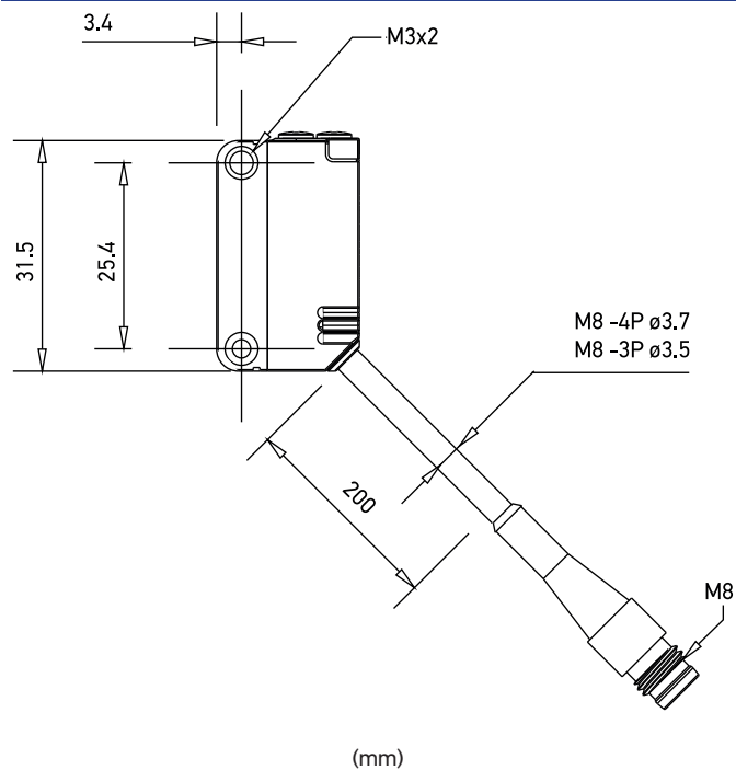
S3N-P*-4-****-**; S3N-P*-6-****-** (M8-4 pins or 3 pins connector pigtail)
