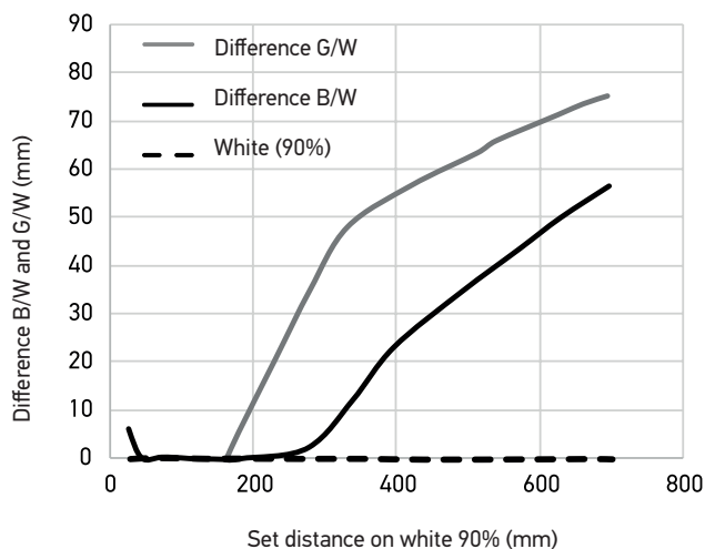
S3N-PH-*-M03-* (Sensing vs. Set Distance difference)
