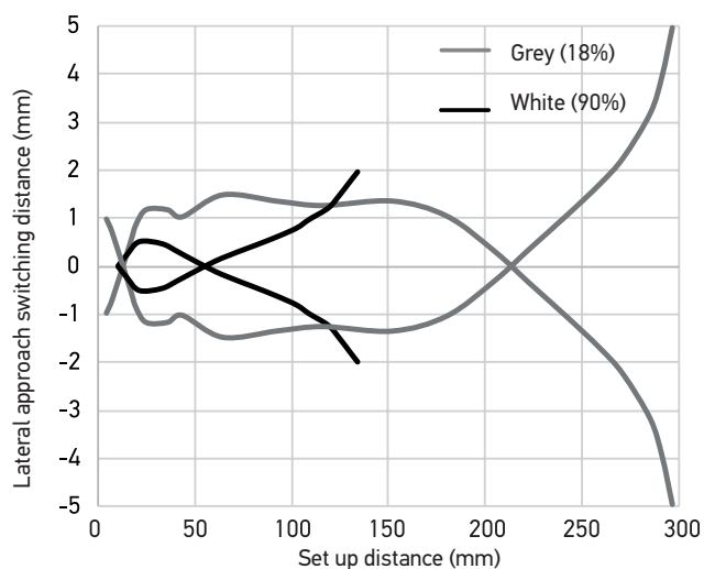
S3N-PR-*-C0*-* (Beam diagram)
