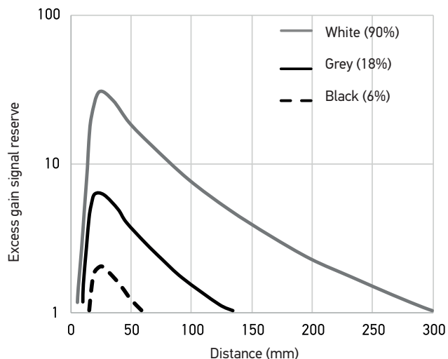
S3N-PR-*-C0*-* (Excess gain)
