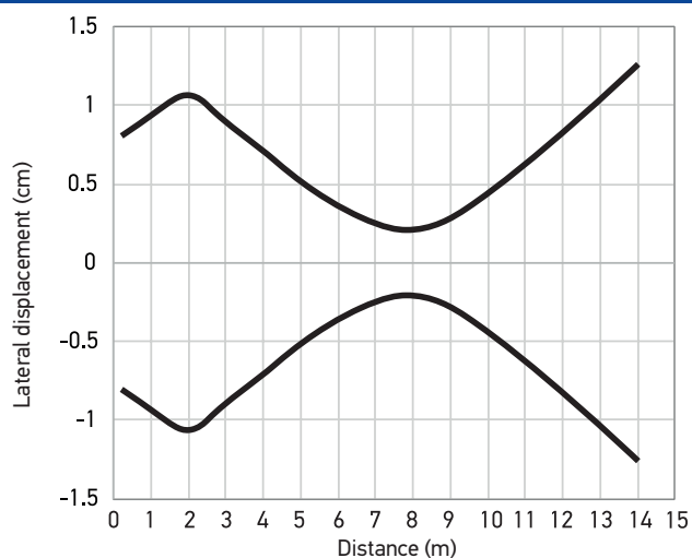
S3N-PH-*-B**-* (Beam diagram)
