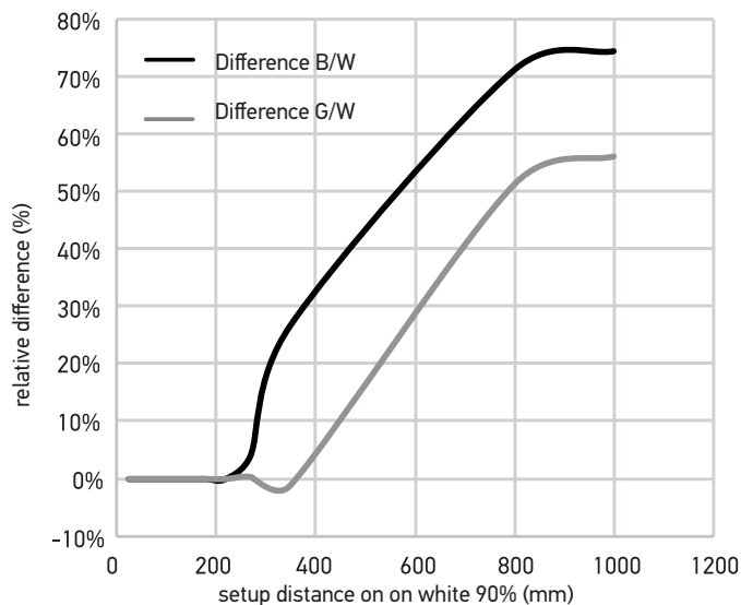
S3N-PR-*-M01-** (Teach behaviour (on white 90%))
